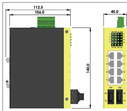
Din-Rail Mount Dimension
