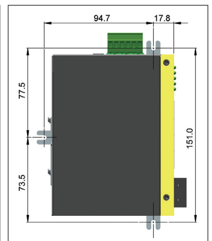
Panel & Wall Mount Dimension
